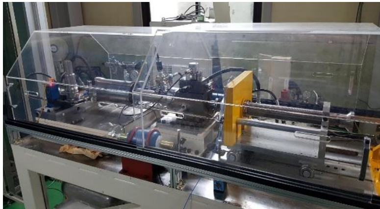
Figure 8 Photograph of servo actuator test equipment
