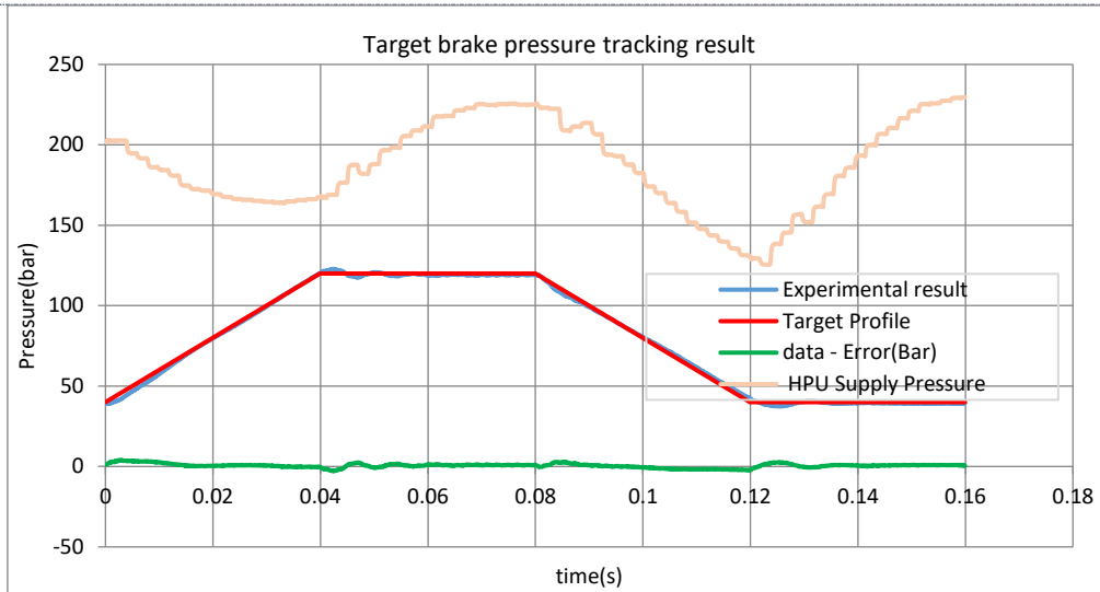
Figure 11 Ramp and step waveform signal tracking of target brake pressure
