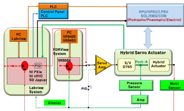
Figure 7 Model Based Tracking Control Algorithm
