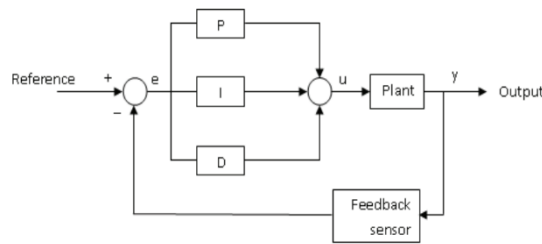
Figure 5 PID algorithm
