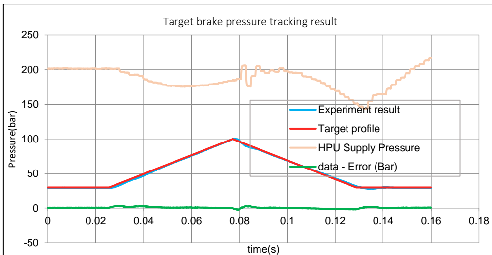
Figure 10 Triangular waveform signal tracking of target brake pressure
